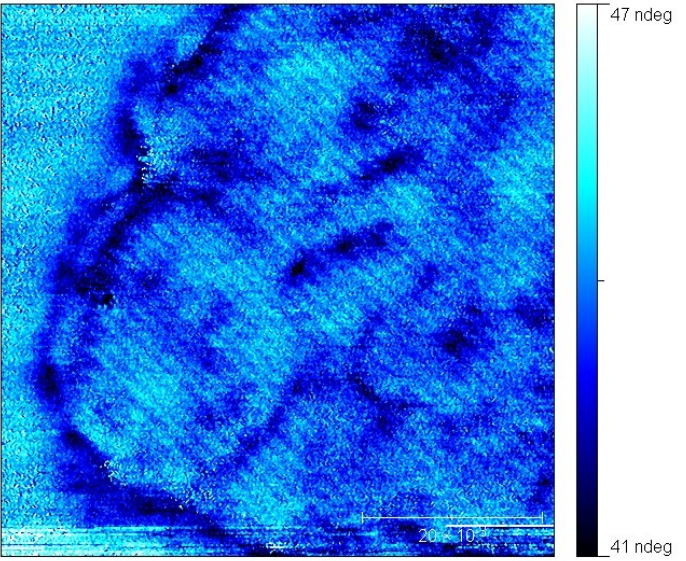
60nm phase scan of dodecylamine on HOPG. The width of lamellae is 1.6 nm.
