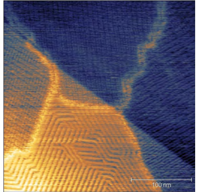
Melissic acid self-assembled on HOPG 325 nm topography
