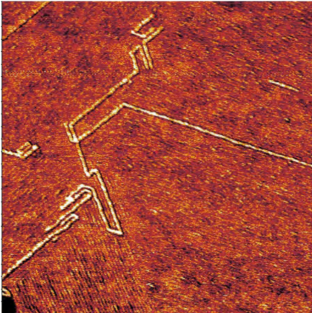
DNA self-assembled on ODA lamellae 500 nm frequency shift image
